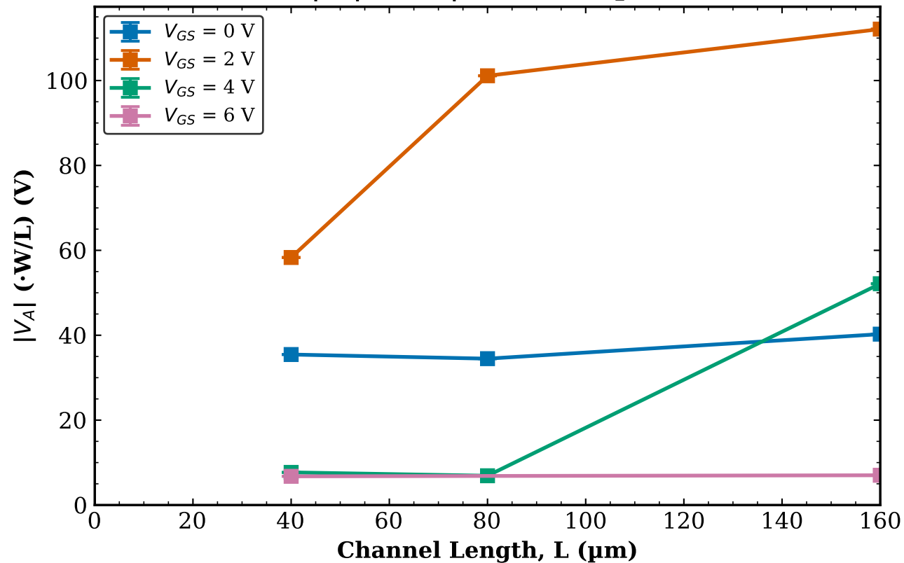
TFT2 Transistor 1 |V_A| vs L | W = 500\text{ }\mu\text{m}
